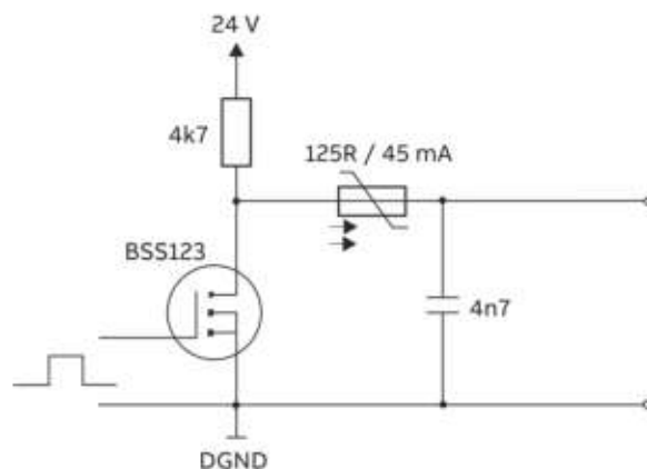
Figure 2: Digital output
